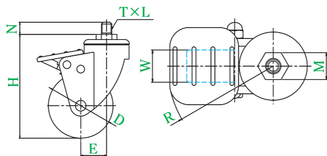
树脂脚轮 \phi 75 M12 \times 14
